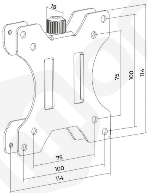
Placa VESA desmontable
